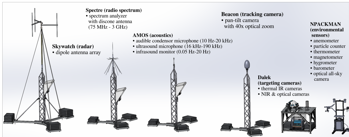
Figure 2. Mechanical designs of the Phase 1 Observatory-class instrumentation suite on the rooftop of the Harvard-Smithsonian Center for Astrophysics (CfA)
