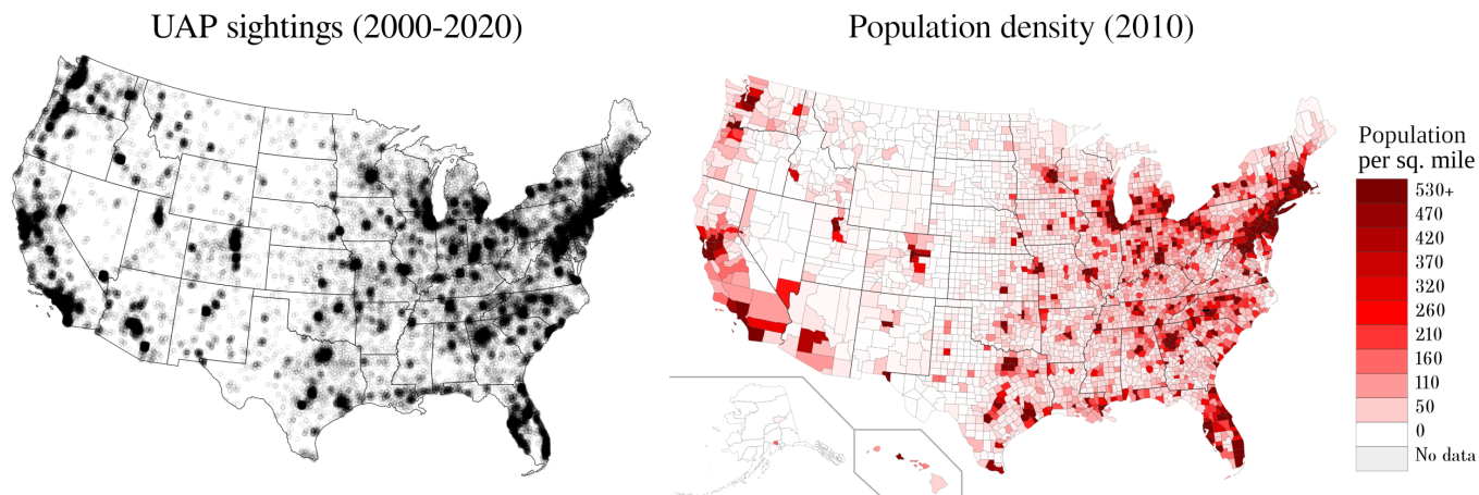
Figure 4. Left: UAP sightings in the continental United States (2000-2020; NUFORC (Davenport 2022)); each circle represents one sighting. Right: Population density (U.S. Census Bureau 2011).
