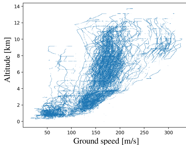
Figure 1. Census of \sim 1200 aircraft whose ground speed and altitude were recorded during a four-day interval in November 2021 over Wellesley, MA, USA. Even this short period and small sample size is sufficient to show the overdense cores of clusters and the emerging boundaries of a performance envelope.
