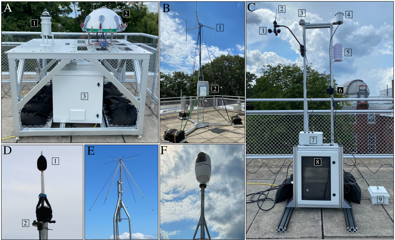
Figure 3. Photographs of Phase 1 Observatory-class instrumentation suite on the rooftop of the CfA. (A) 1. ALCOR OMEA 9C all-sky camera; 2. Dalek hemispherical array of 8 LWIR microbolometer cameras (covered) and single optical + near-infrared all-sky camera; 3. Weatherproof enclosure for instrument computers. (B) SkyWatch radar tower: 1. dipole antenna array; 2. electronics enclosure. (C) NPACKMAN environmental monitoring system: 1. anemometer; 2. wind vane; 3. rain sensor; 4. optical all-sky camera; 5. temperature and pressure sensors; 6. camera fuse/switch box; 7. scintillation particle counter; 8. power and data module; 9. fluxgate magnetometer. (D) 1. GRAS audible microphone; 2. Wildlife Acoustics ultrasound microphone; infrasonic sensor not shown. (E) Discone wide-band antenna for spectrum analyzer (Spectre). (F) Beacon 8 narrow-field pan-tilt-zoom camera.
